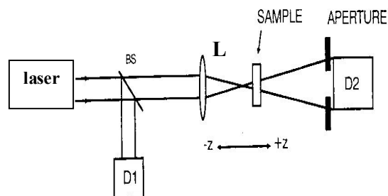
Fig. (1): Schematic diagram of a single beam z-scan setup: L: Lens; S: Sample; A: Aperture; D 1 , D 2 : Detectors; BS: Beam Splitter
