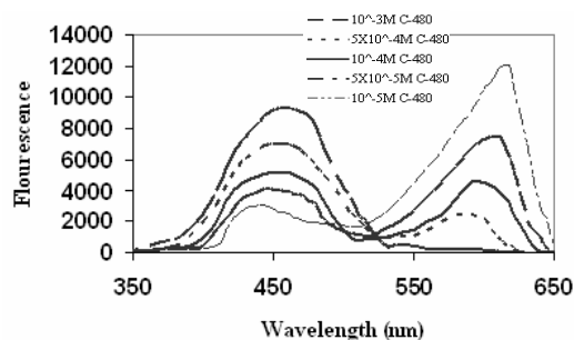
Fig. (4): The fluorescence spectra of mixed laser dyes at 10^{-4} M of Rh-6G.
