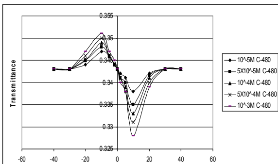
Fig. (5): closed aperture z-scan of mixture laser dyes at 10^{-4} M of Rh-6G at
