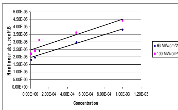
Fig. (10): Nonlinear absorption of different concentration of donor at 100 MW/cm 2 and 63 MW/cm 2 power densities
