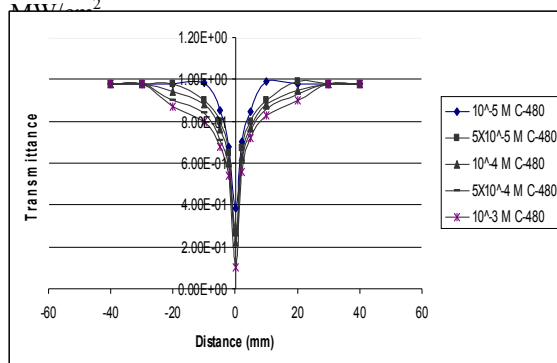
Fig. (8): open aperture z-scan of different concentration of donor at 10 -4 M acceptor at 63 MW/cm 2
